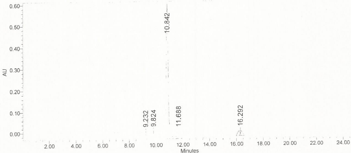
Auto-Scaled Chromatogram
